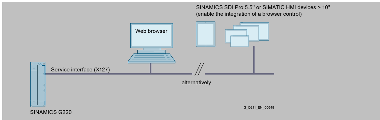
Integration of the SINAMICS web server based on the example of a SINAMICS G220 and the service interface (X127)
