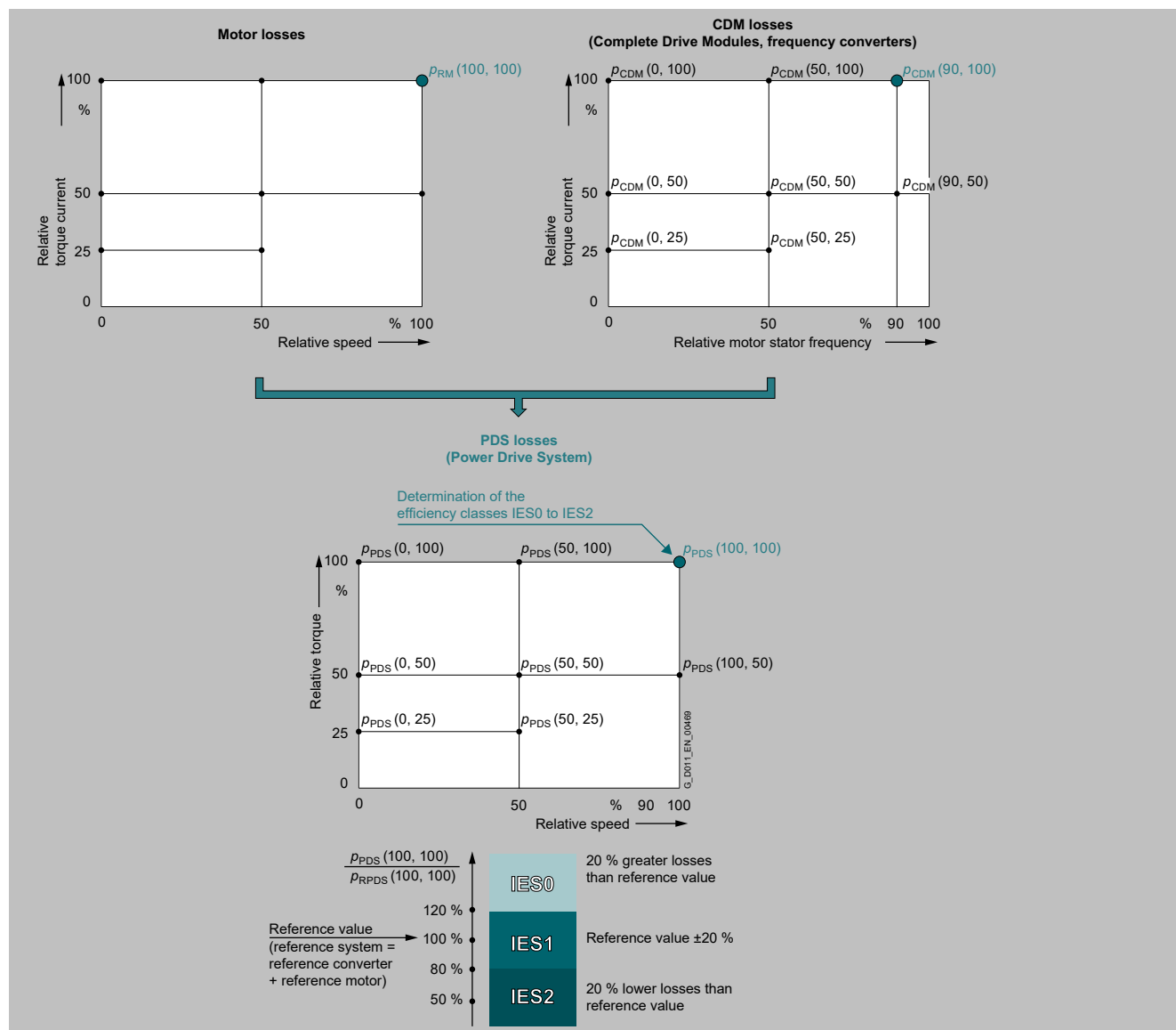
Power Drive System (PDS) – determining the efficiency class
