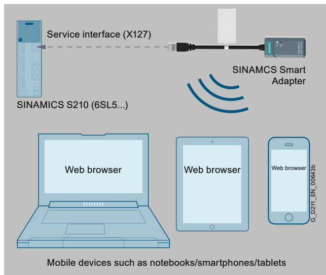
Wireless access to the web server via the service interface (X127) of the SINAMICS S210 (6SL5...) with the help of the SINAMICS Smart Adapter
