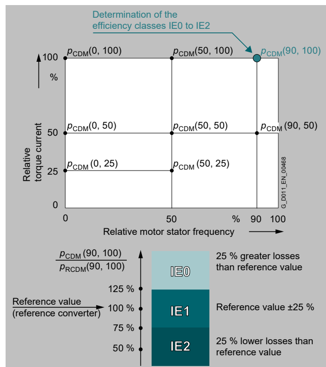
Complete Drive Module (CDM) – determining the efficiency class
