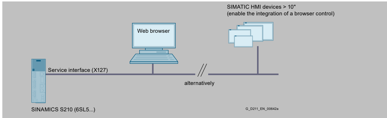
Integration of the SINAMICS web server based on the example of a SINAMICS S210 (6SL5...) and the service interface (X127)
