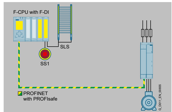
Integrated safety via PROFIsafe
