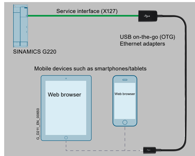
Access to the web server via the service interface (X127) of the SINAMICS G220 with the help of a USB on-the-go (OTG) Ethernet adapter
