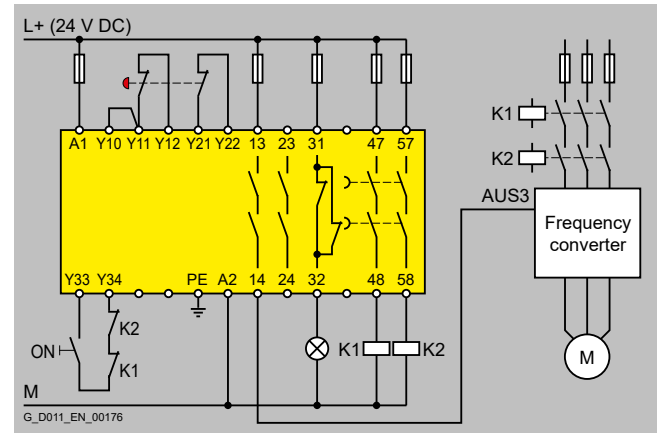
Classic implementation using an external circuit
