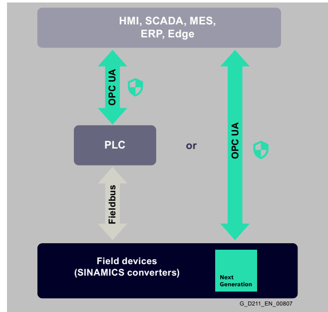
Topology SINAMICS OPC UA
