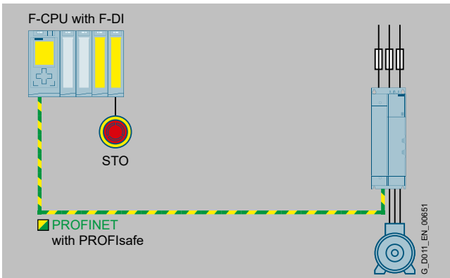
Integrated safety via PROFIsafe
