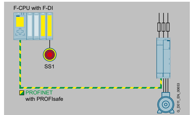
Integrated safety via PROFIsafe
