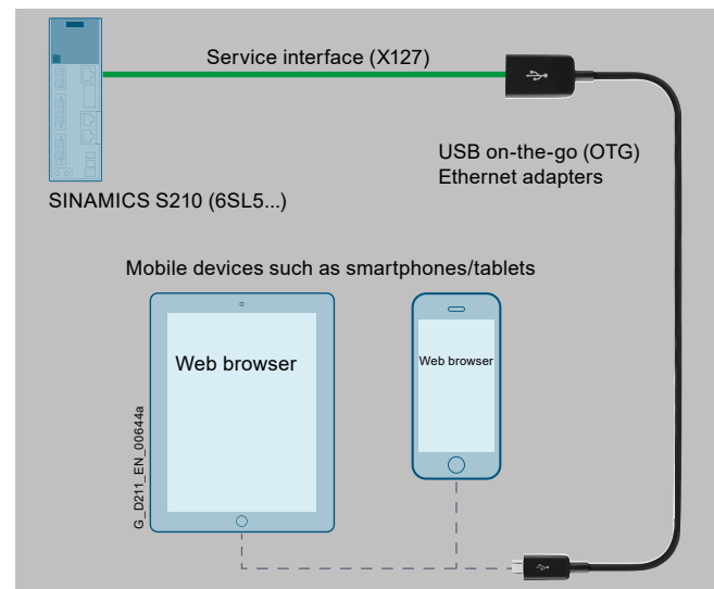
Access to the web server via the service interface (X127) of the SINAMICS S210 (6SL5...) with the help of a USB on-the-go (OTG) Ethernet adapter
