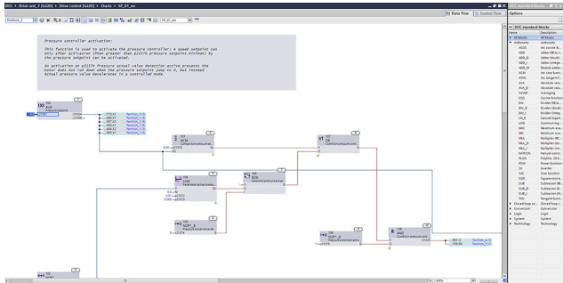
SINAMICS DCC (Drive Control Chart) - example with a servo pump application for next generation of SINAMICS converters
