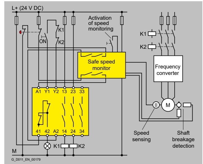
Classic implementation using an external circuit
