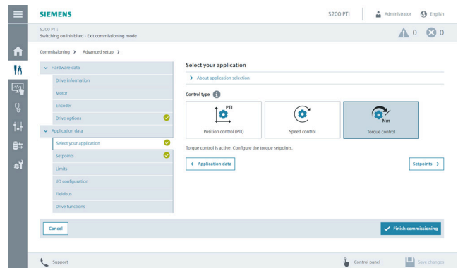
Advanced commissioning of SINAMICS S200, Pulse Train Input version (PTI), with open dialog for application selection
