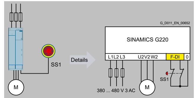
Standalone safety solution via fail-safe inputs
