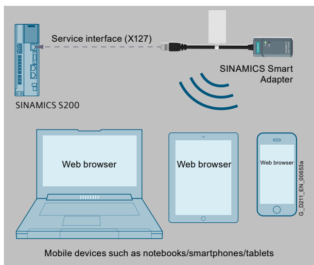
Wireless access to the web server via the service interface (X127) of the SINAMICS S200 with the help of the SINAMICS Smart Adapter
